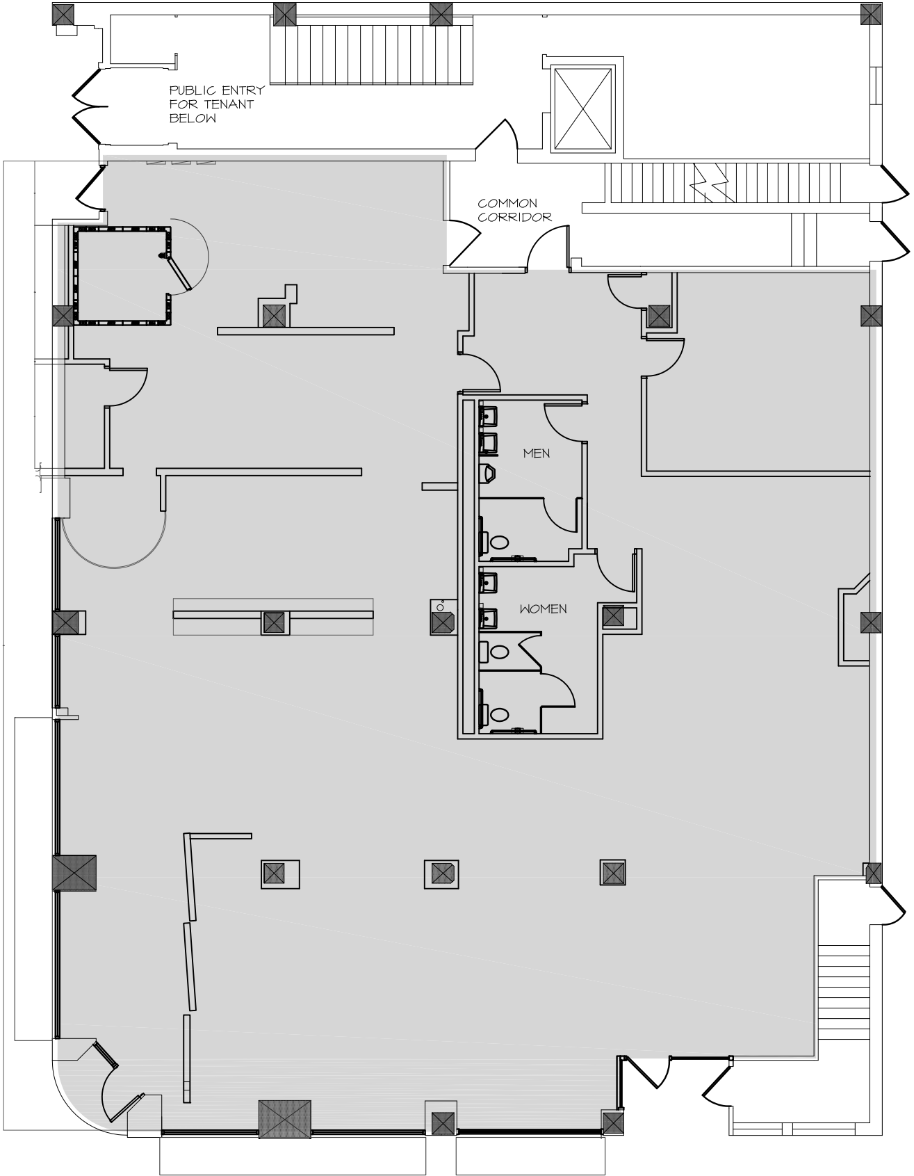
250 State Street First Floor Plan
